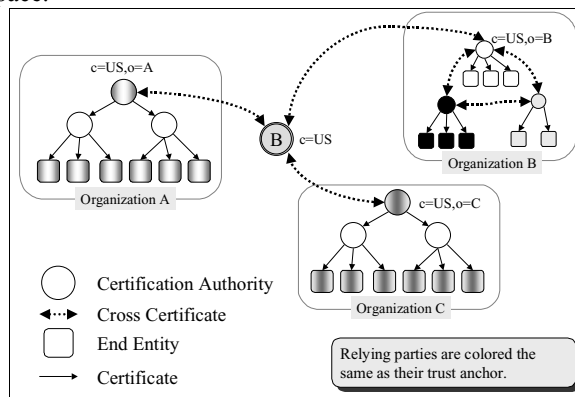
Figure 6: Name Constraints with a Bridge CA
