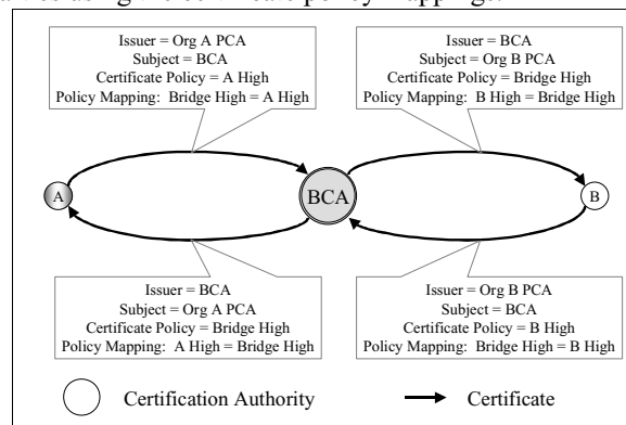
Figure 7: Policy Mapping with a Bridge CA
