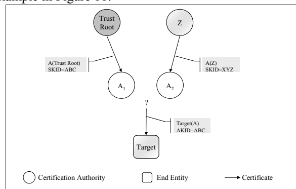
Figure 11: Key Identifier Example
